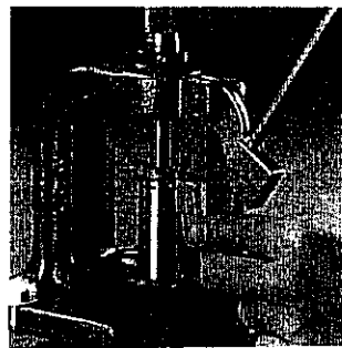
Push the primer arm forward and lower the press handle.
