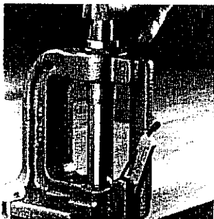
Lower the press handle and install the swager assembly.
